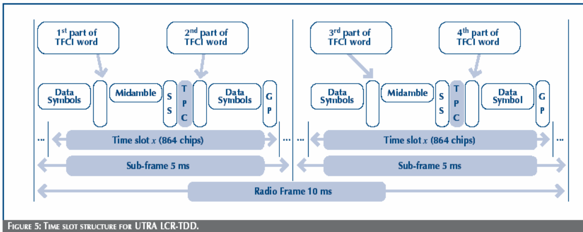
FIGURE 5: TIME SLOT STRUCTURE FOR UTRA TCR-TDD.
