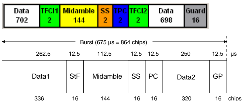
Fig. 5 Traffic burst with layer 1 control information
