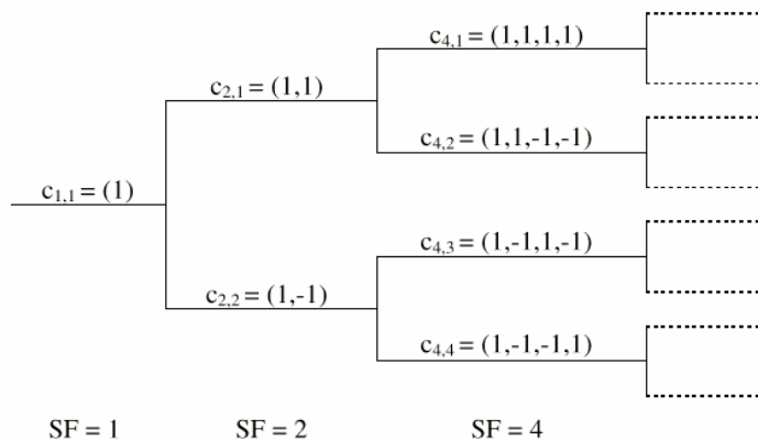
Code tree of channelization codes
