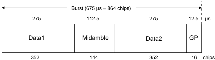
Fig. 4 Traffic burst without layer 1 control information
